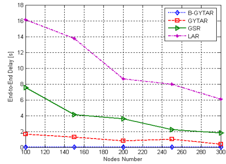
Figure 7 –End-to-End Delay Vs Nodes Number (5 packets/ second).
